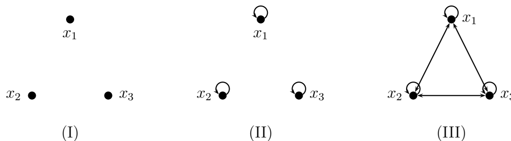
Figure 8.1: Binary Relations
