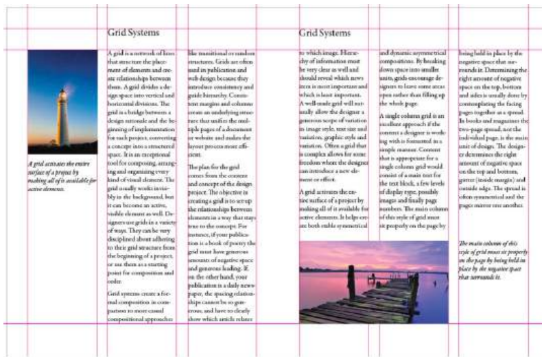
Figure 3.32 Multi-column grid
