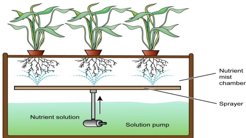
Fig. 2.3: An Aeroponic Growth System (Based on Taiz et al)
