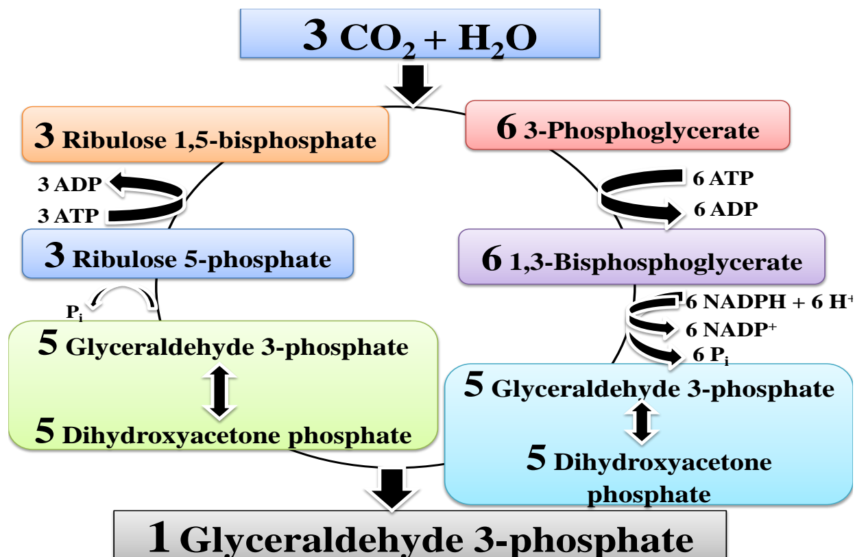
Figure 4.8: The \text{CO}_2 assimilation in the Calvin or \text{C}_3 cycle.
