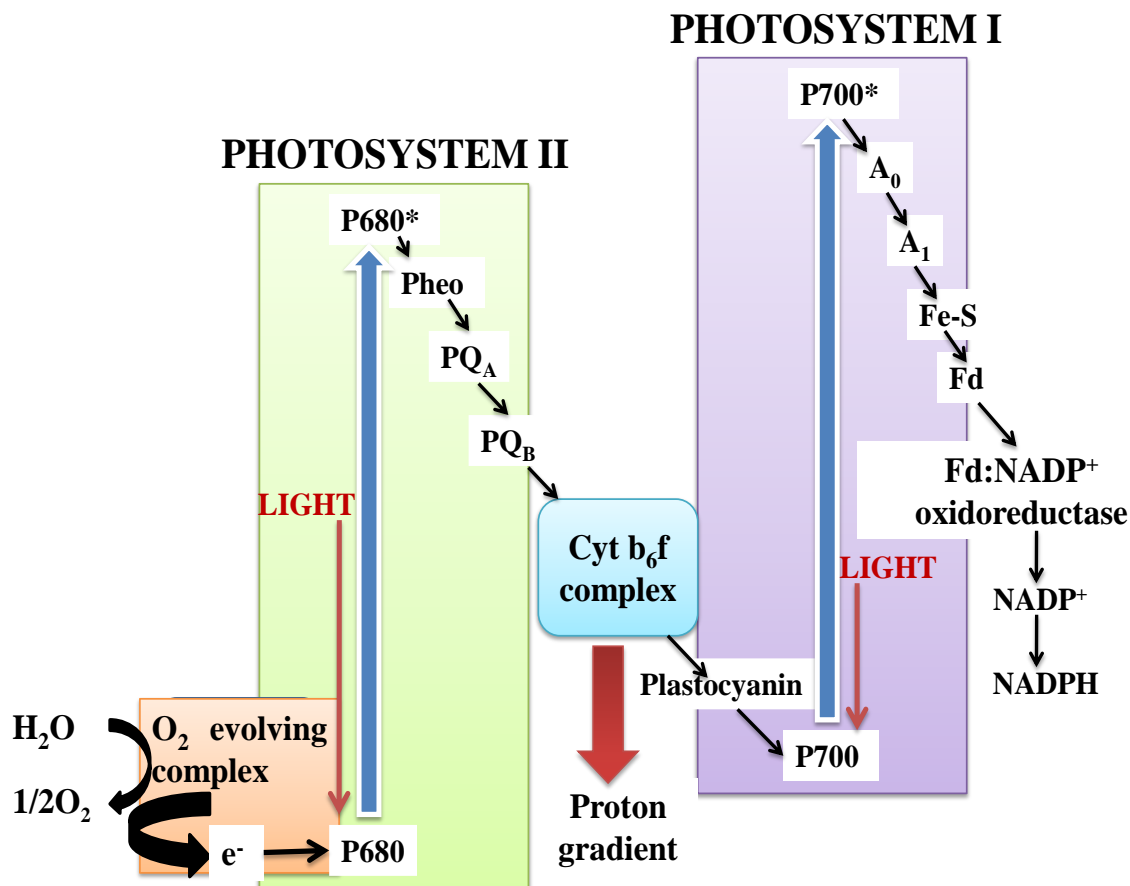
Figure 4.3: Photosystem I and Photosystem II in the Z-scheme of Chloroplast.
