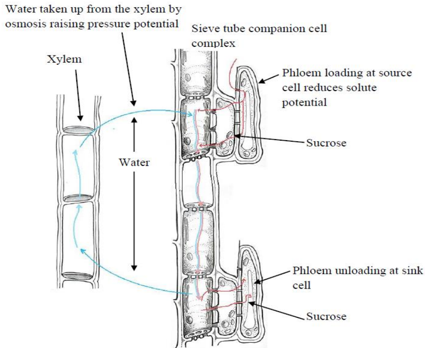
Figure. 3.3. Mechanism of phloem transport
