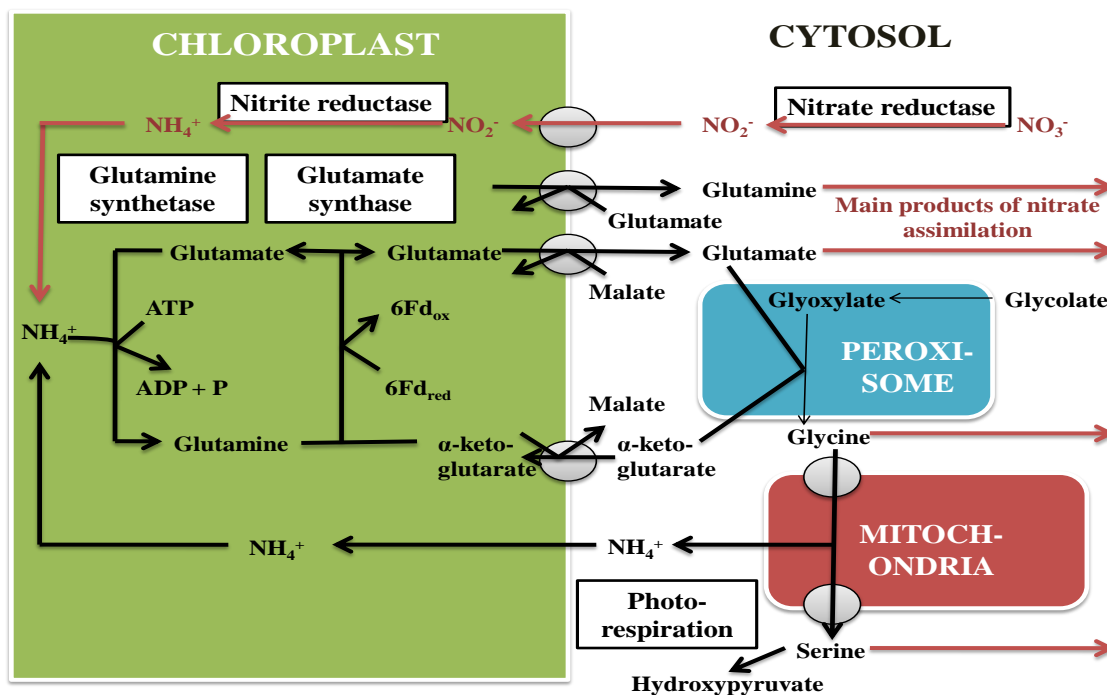
Figure 6.7: The production of main products of nitrate assimilation.
