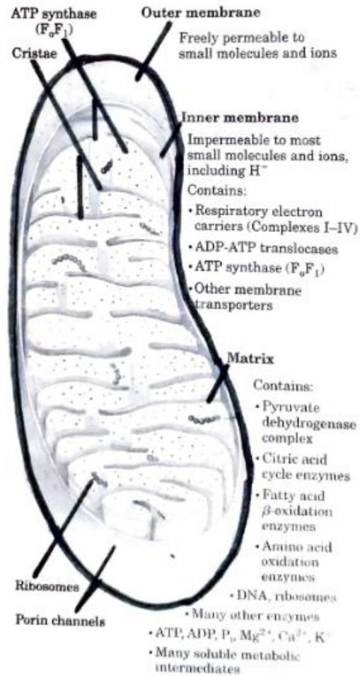
Fig:5.3. Biochemical anatomy of mitochondria
