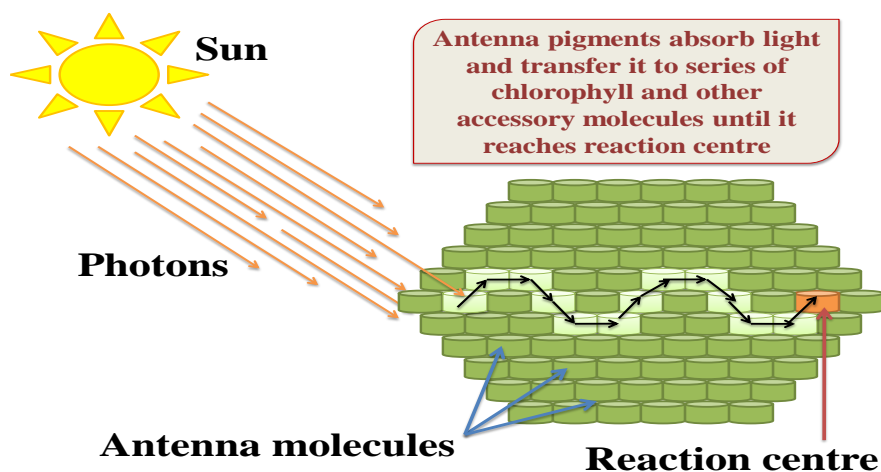
Figure4. 2: The diagrammatic representation of photosynthetic units.
