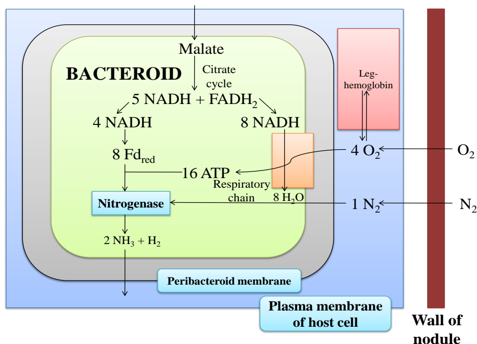
Figure 6.4: The process of nitrogen fixation in bacteroids.
