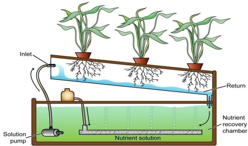
Figure. 2.2: A Nutrient film growth System (Based on Taiz et al)
