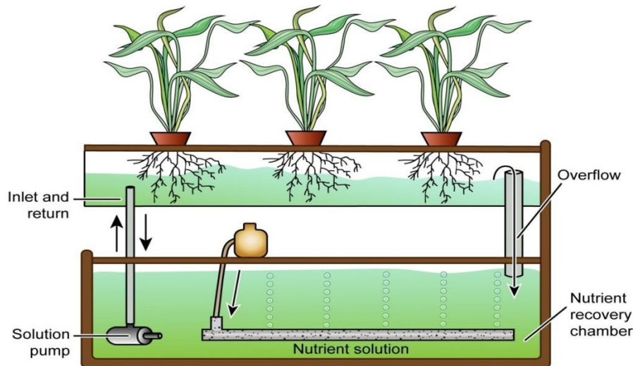
Fig.2.4: An Ebb and Flow system ((Based on Taiz et al)
