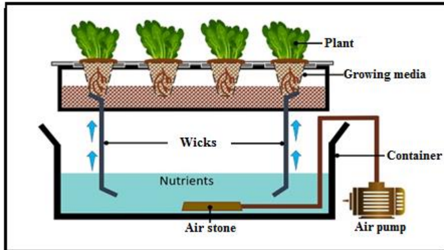
Fig.2.6: Wick System (Source- Google images)
