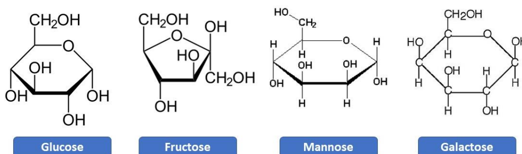
Fig. 8.3: Structure of some common hexose sugar
