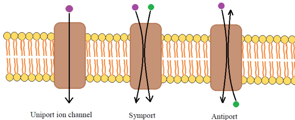
Fig 3.1. Transport of ions across the membrane
