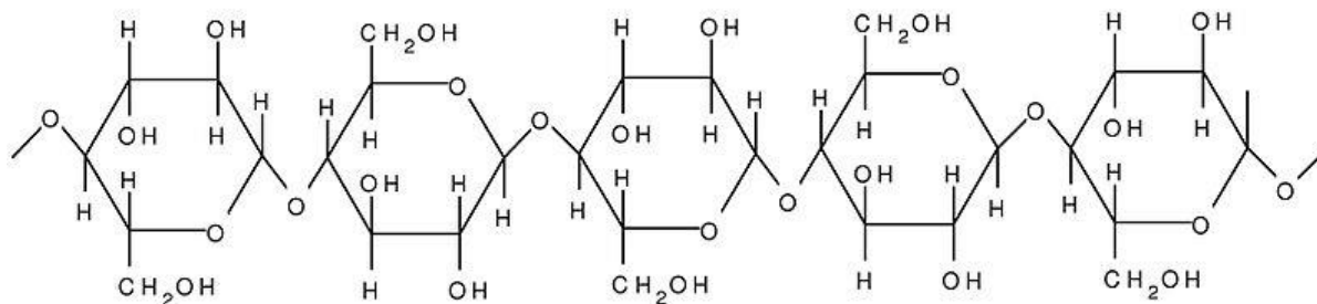
Figure 8.8. Structure of cellulose
