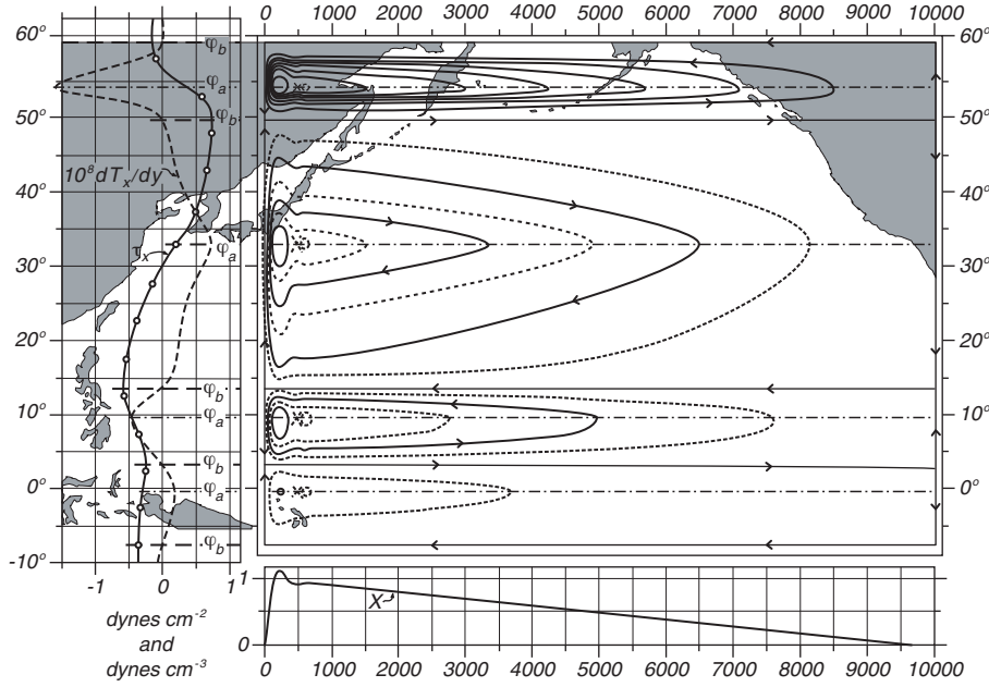
Figure 11.6 Left: Mean annual wind stress T_x(y) over the Pacific and the curl of the wind stress. \varphi_b are the northern and southern boundaries of the gyres, where M_y = 0 and \text{curl } \tau = 0 . \varphi_0 is the center of the gyre. Upper Right: The mass transport stream function for a rectangular basin calculated by Munk (1950) using observed wind stress for the Pacific. Contour interval is 10 Sverdrups. The total transport between the coast and any point x, y is \psi(x, y) . The transport in the relatively narrow northern section is greatly exaggerated. Lower Right: North-South component of the mass transport. After Munk (1950).
