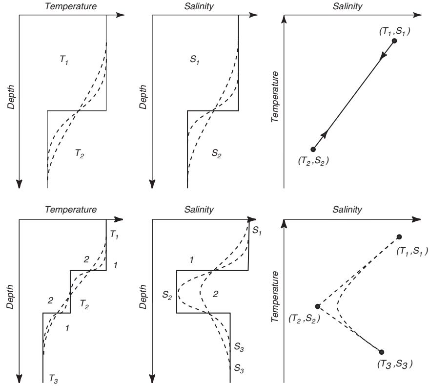
Figure 13.7 Upper: Mixing of two water masses produces a line on a T-S plot. Lower: Mixing among three water masses produces intersecting lines on a T-S plot, and the apex at the intersection is rounded by further mixing. After Defant (1961: 205).
