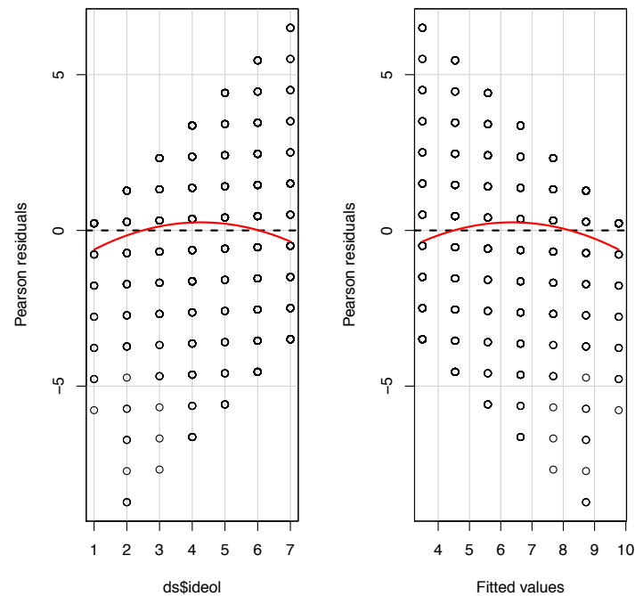
Figure 10.7: Residual Plots Examining Model Linearity
