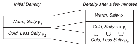
Figure 8.8 Left: Initial distribution of density in the vertical. Right: After some time, the diffusion of heat leads to a thin unstable layer between the two initially stable layers. The thin unstable layer sinks into the lower layer as salty fingers. The vertical scale in the figures is a few centimeters.
