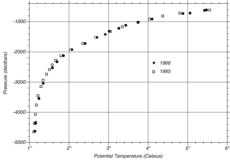
Figure 8.4 Potential temperature measured as a function of depth (pressure) near 24.7^{\circ}\text{N} , 161.4^{\circ}\text{W} in the central North Pacific by the Yaquina in 1966 ( \bullet ), and by the Thompson in 1985 ( \square ). Data from Atlas of Ocean Sections produced by Swift, Rhines, and Schlitzer.
