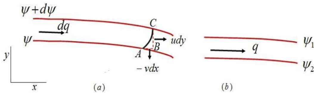
Fig. Flow between two streamlines
