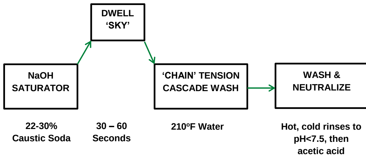
Figure 5 - Schematic of the Mercerization Process.
