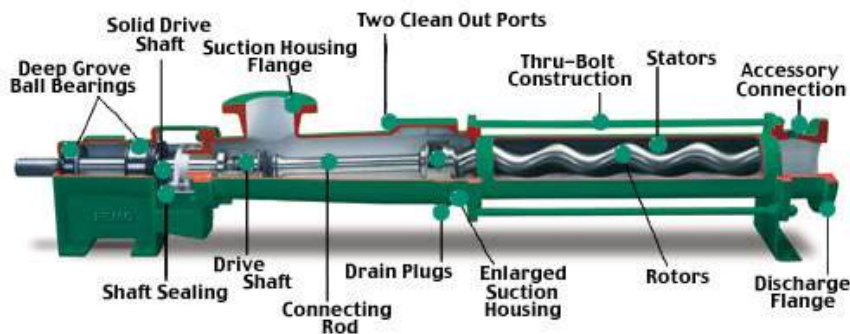
FIGURA 8.3: Bomba helicoidal.
