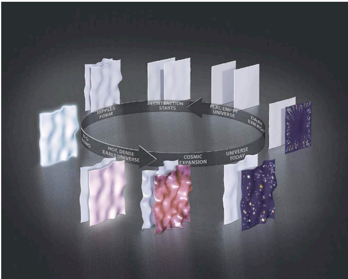
The Steinhardt-Turok Cyclical Multiverse (8)
