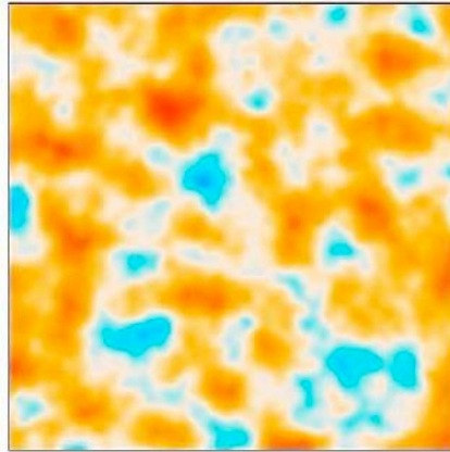
WMAP
