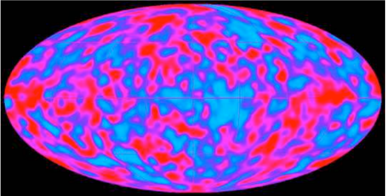
COBE All-Sky Map 1992
