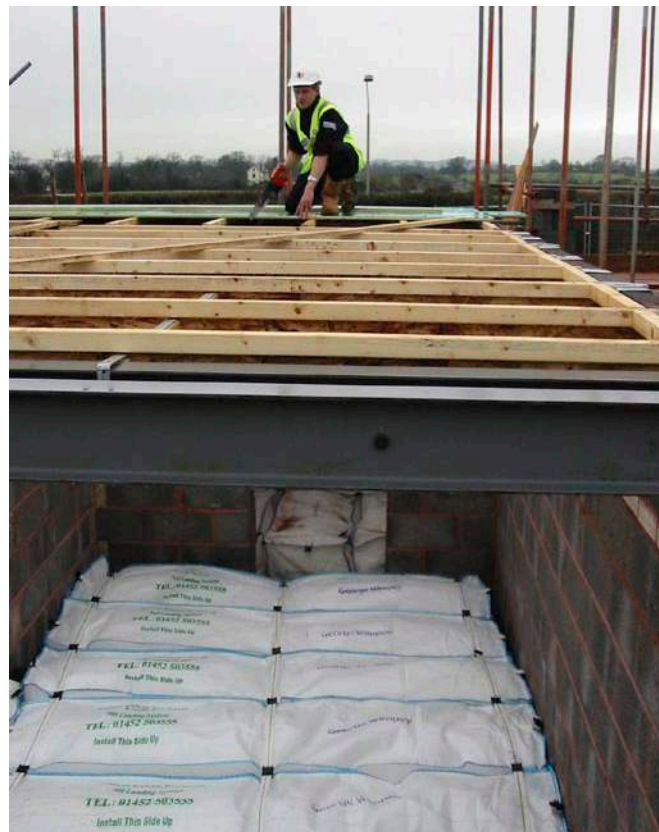
Figure 15 Soft landing system
