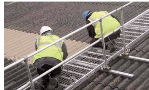
Figure 27 Workmen wearing harnesses attached to a work positioning line, which is fitted to the staging
