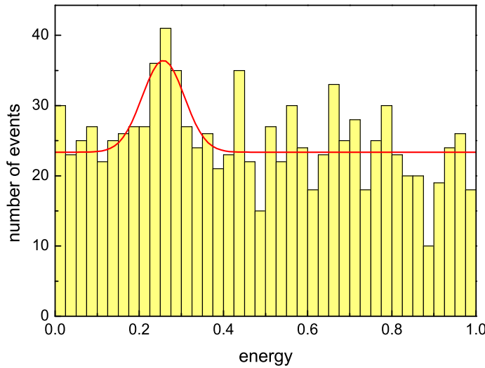
Fig. 10.18. Histogram of event sample used for the likelihood ratio test. The curve is an unbinned likelihood fit to the data.
