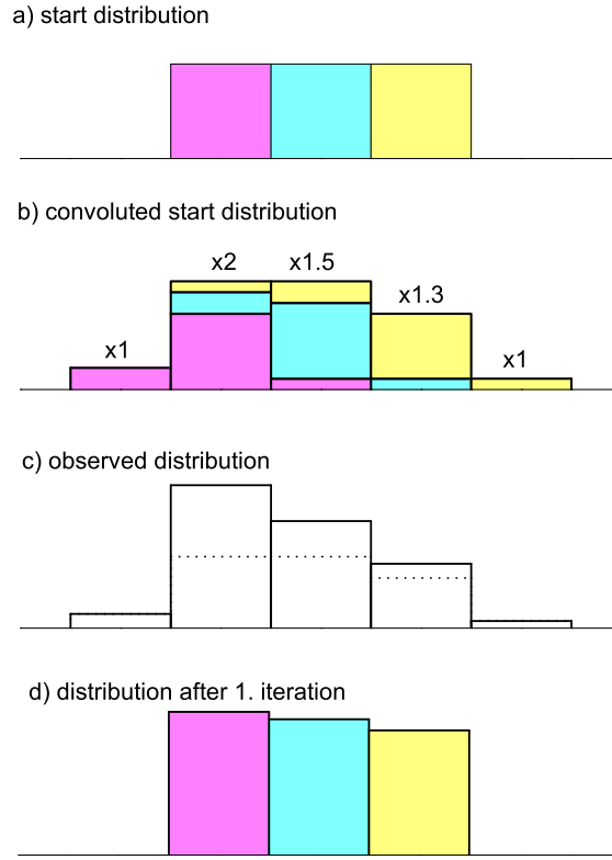
Fig. 9.5. Iterative deconvolution.
