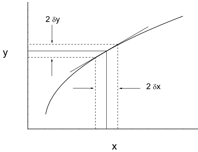
Fig. 4.1. Linear error propagation.
