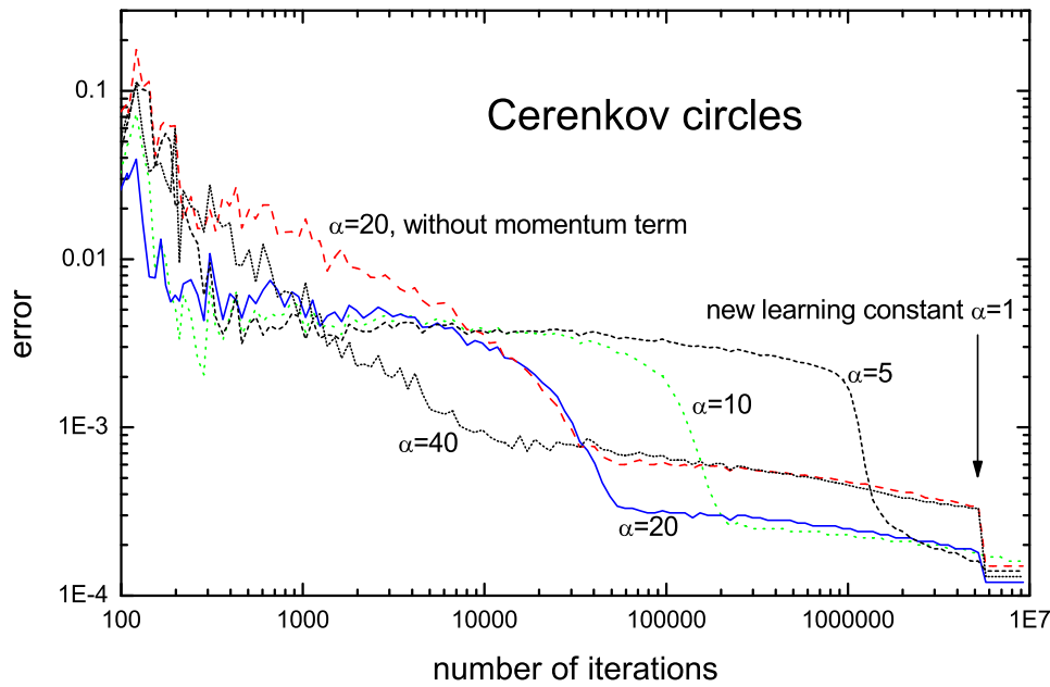
Fig. 11.11. Reconstruction of radii of circles through 5 points by means of an ANN with different sequences of learning constants \alpha .
