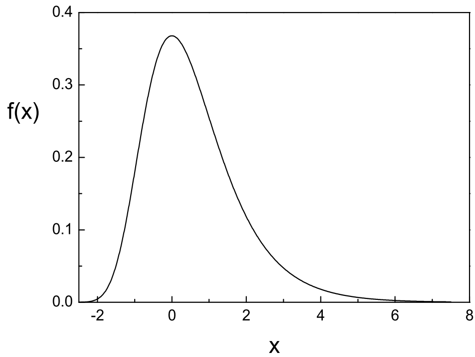
Fig. 3.24. Log-Weibull distribution.
