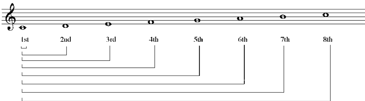
The notes in the C major scale form these intervals above the tonic (C)
