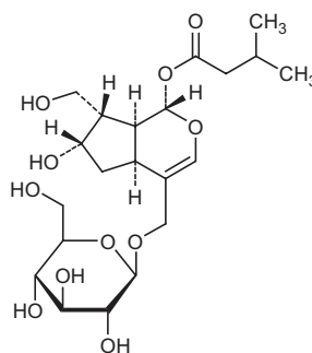
Patrinoside
