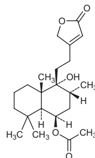
Vitexilactone
