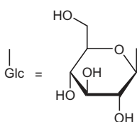
β-D-glucopyranosyl
