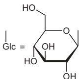
\beta -D-glucopyranosyl
