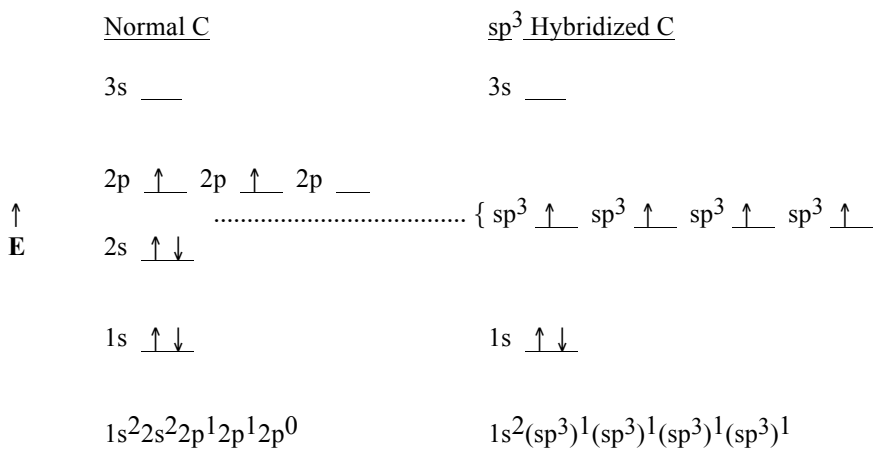
Figure [graphic 1.35]. Electron Energy Diagrams for Ground State and sp^3 Hybridized C.
