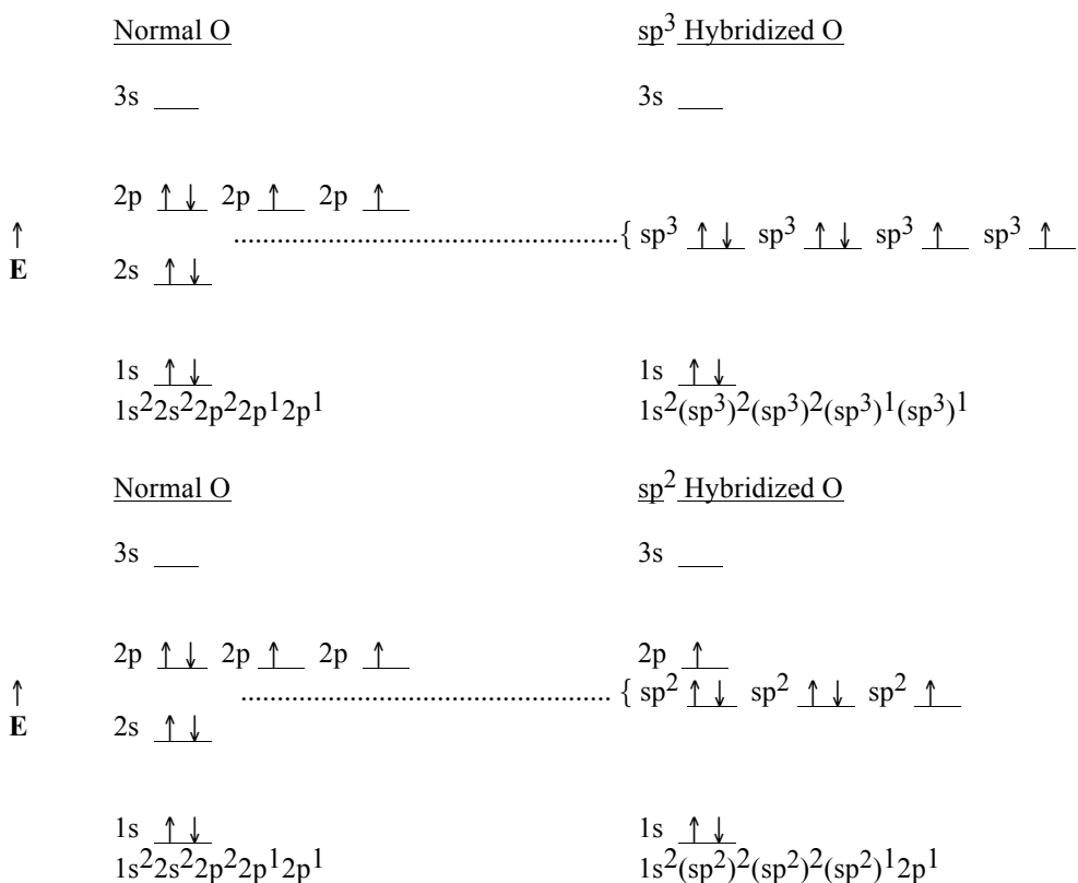
Figure [graphic 1.62]. Electron Energy Level Diagrams for Ground State, sp 3 , and sp 2 Hybridized O
