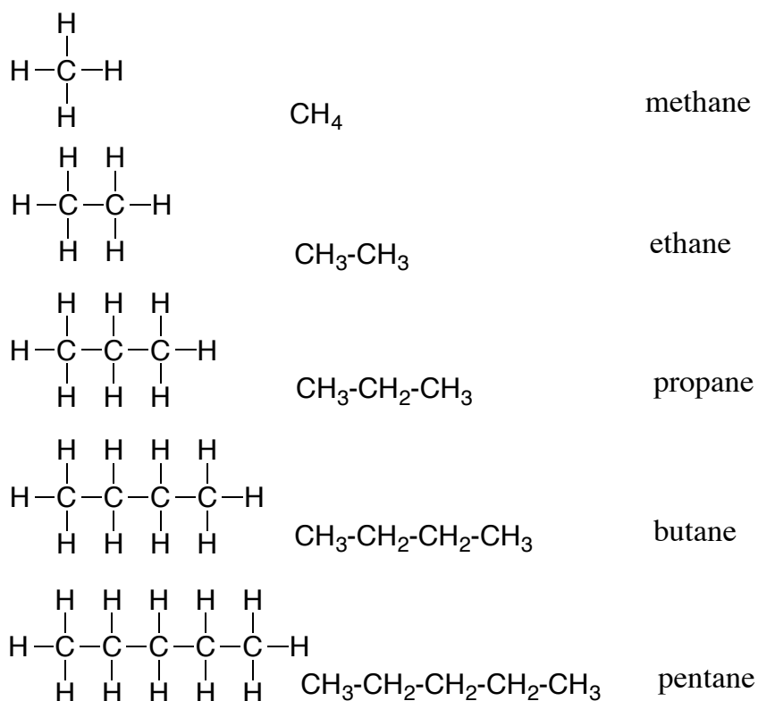
Fig. 1.7 Linear Alkanes
