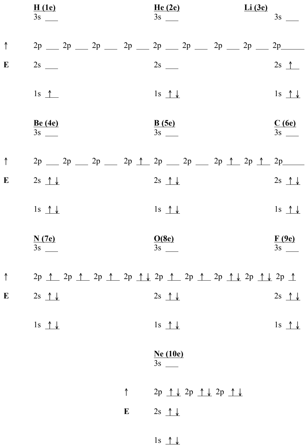
Figure [graphic 1.26]. Electron Energy Diagrams for The First Ten Elements
