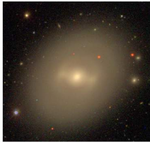
Fig 1.13 (Hogg, Blanton, SDSS) 'Galaxies in the Universe' Sparks/Gallagher CUP 2007
