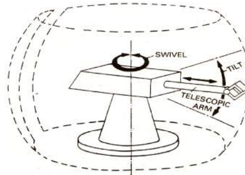
Fig. 10.5 Spherical Workspace Configuration
