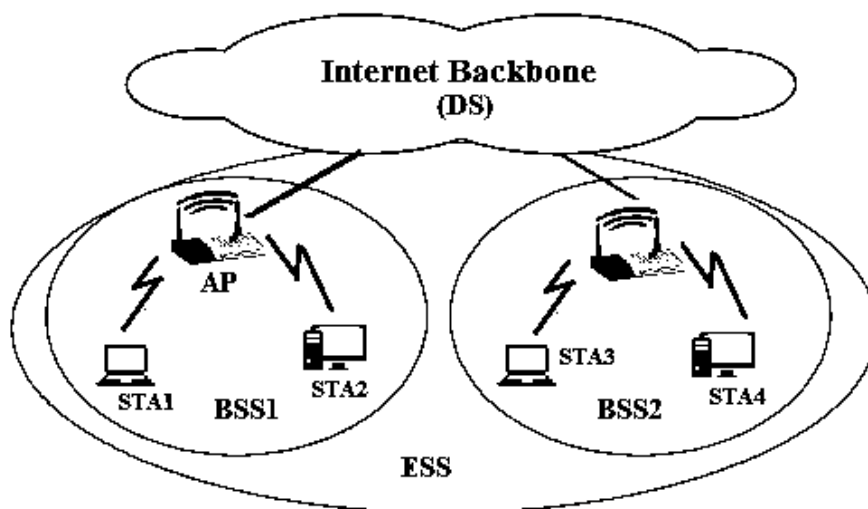
Figure 30: 802.11 components.
