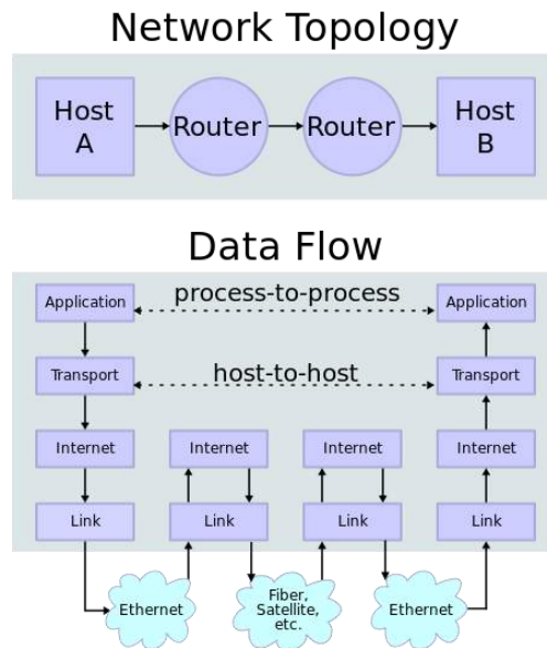
Figure 27: Internetworking.
