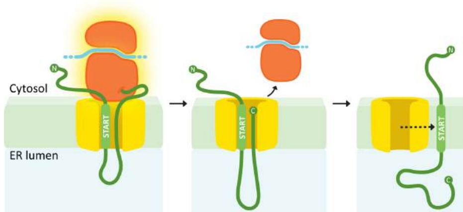
Figure 04-09: Insertion of a protein with one internal START sequence. This image was created by Heather Ng-Cornish and is shared under a CC BY-SA 4.0 license.
