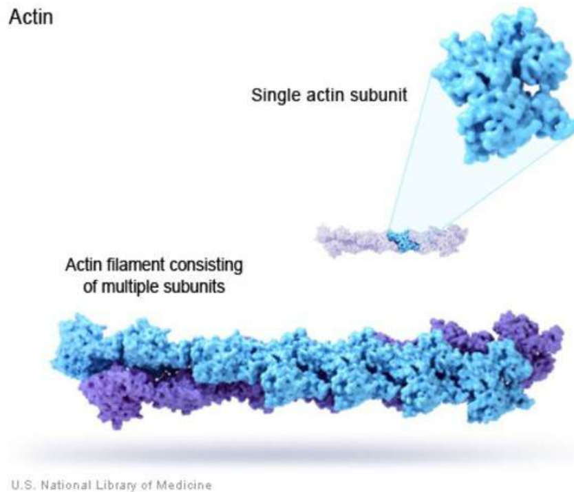
Figure 06-18: The molecular structure of actin filaments. Actin proteins polymerize into a filament with a twisted shape. Image source: MedlinePlus , National Library of Medicine. This image is in the public domain.
