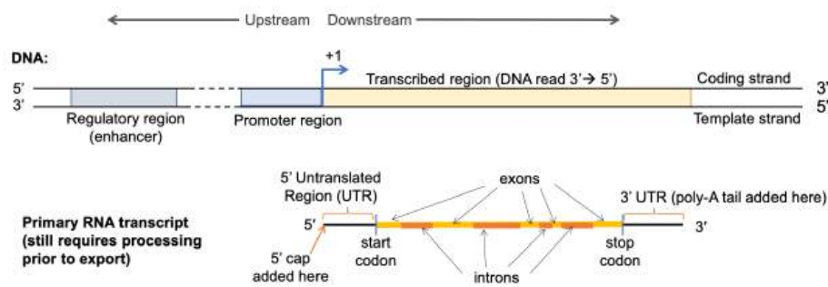
Figure 03-10: The structure of a eukaryotic gene (top) and its relationship to the transcribed mRNA (bottom). This image was created by Dr. Robin Young and is shared under a CC BY-SA 4.0 license.
