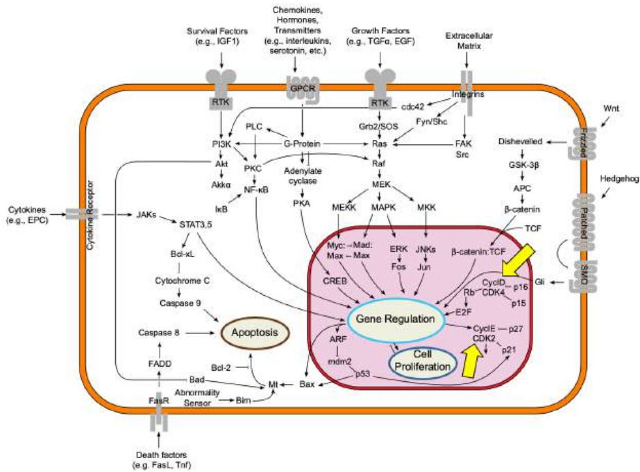
Figure 08-04: CDK2 (and its cyclin, CyclE) and CDK4 (+CyclD) within the signaling cascade that controls growth proliferation and/or apoptosis. “Signal Transduction pathways” by BohHog2 modified by Dr. Robin Young . This image is in the public domain .
