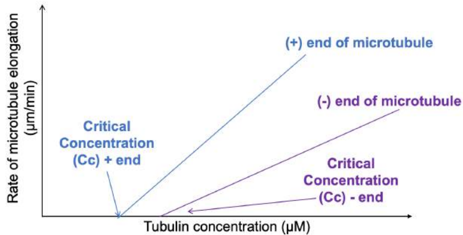
Figure O6-11: The rate of reaction is dependent on the concentration of the tubulin subunits available. The higher the concentration of tubulin subunits, the higher the rate of assembly. Notice also that the rate of assembly is always slower on the minus end of the polymer. On the plus end of microtubules, fewer subunits are needed (lower concentration) to begin filament formation. Graph is based on data from Walker et al. (1988) . Image by Dr. Robin Young is licensed under CC BY-SA 4.0 .
