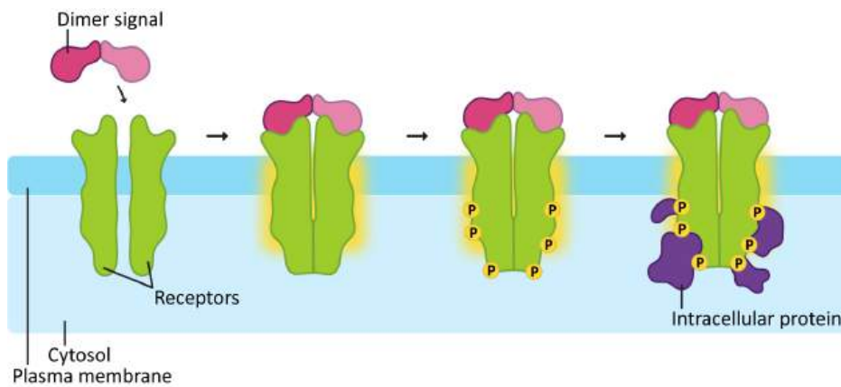
Figure 07-12: Activation of receptor tyrosine kinases. The ligand is a dimer (shown in pink) and binds to the receptor on the extracellular side, causing two receptors to dimerize, cross phosphorylate, and activate. Phosphorylation creates docking sites, allowing for recruitment of other enzymes and downstream signaling targets. This image was created by Heather Ng-Cornish and is shared under a CC BY-SA 4.0 license.
