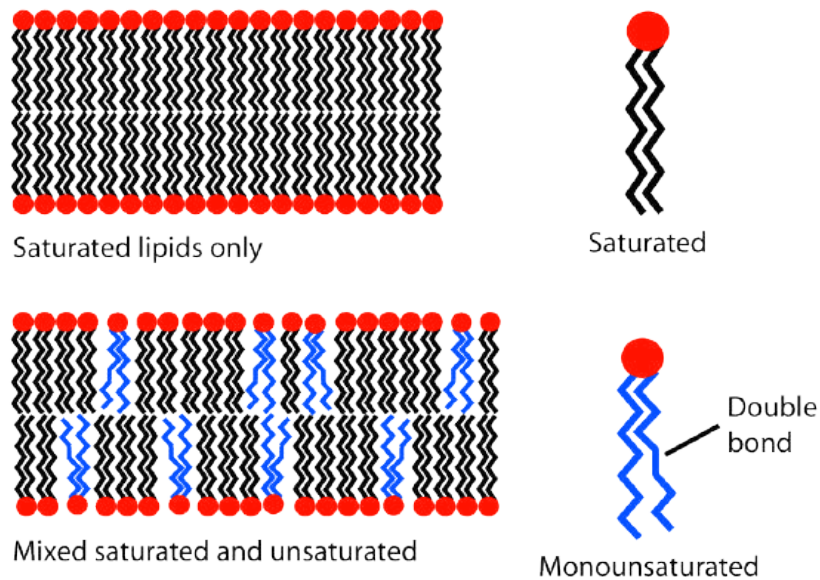
Figure O2-08: Depiction of how unsaturated phospholipids can impact the packing of lipids in a bilayer. Lipid unsaturation effect.svg by MDougM. This image is in the public domain.
