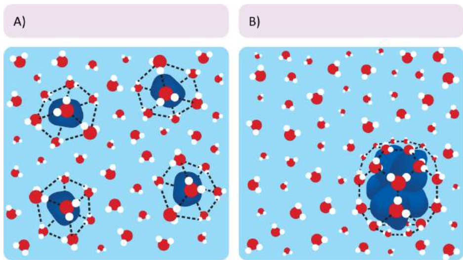
Figure 02-04: Nonpolar molecules clump together in aqueous solution. (A) several nonpolar molecules are in aqueous solution. Water molecules around a nonpolar particle form a cage-like structure, which reduces their motional freedom. (B) The nonpolar molecules are clumped together. This allows more water molecules to be free and engaged in the cage-like hydration shell outside of the nonpolar particle. This image was created by Heather Ng-Cornish and is shared under a CC BY-SA 4.0 license.
