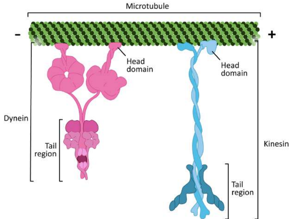
Figure 06-17: Structural representations of kinesin and dynein on a microtubule. The head domain binds to the microtubule reversibly (in an ATP-dependent manner). Through cycles of ATP hydrolysis, these motors are able to walk along the microtubule in a specific direction. This image was created by Heather Ng-Cornish and is shared under a CC BY-SA 4.0 license.
