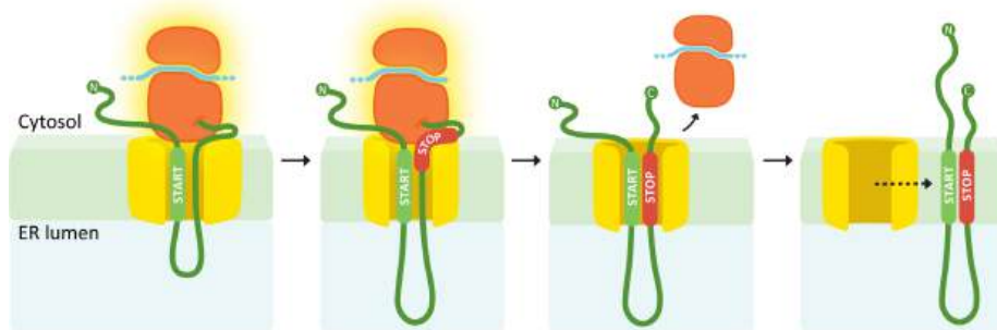
Figure 04-11: A protein with two transmembrane domains that has been inserted into the membrane. This image was created by Heather Ng-Cornish and is shared under a CC BY-SA 4.0 license.
