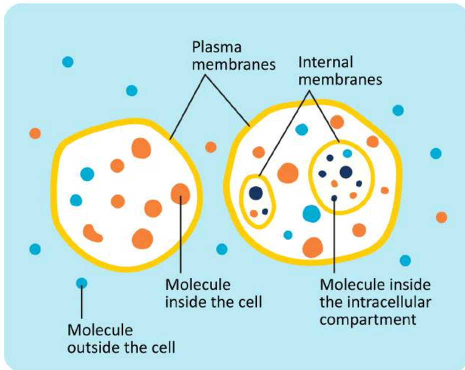
Figure 02-01: Biological membranes act as barriers and separate molecules (represented as colored blobs) into different compartments. This image was created by Heather Ng-Cornish and is shared under a CC BY-SA 4.0 license.
