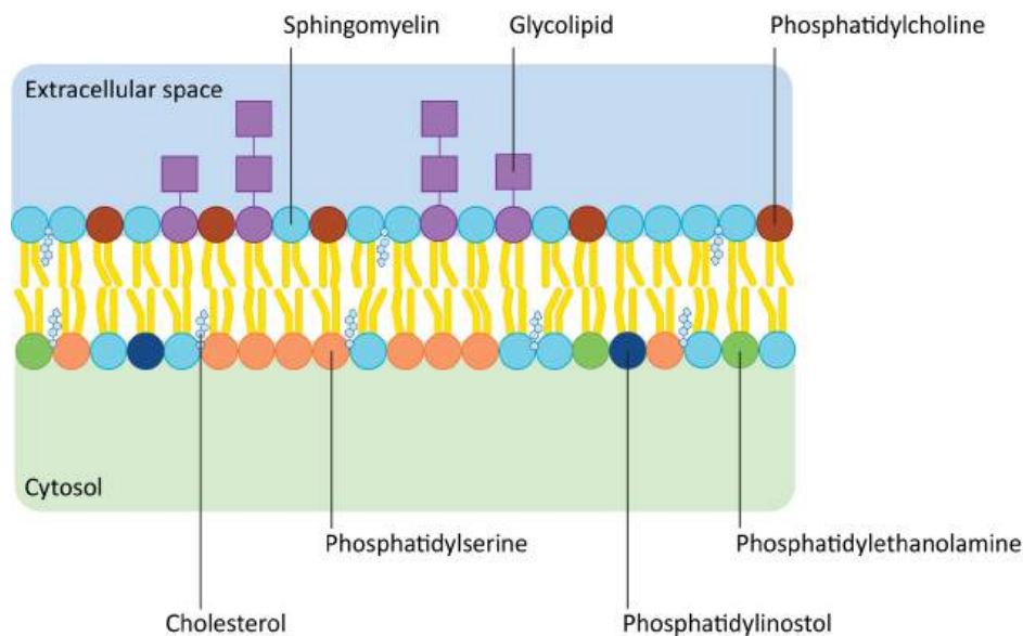
Figure 02-06: The composition of lipids in the biological membrane is distinct and asymmetric. This schematic of a plasma membrane clearly shows differences in the lipids on each side of the membrane. On the exterior side, which faces the extracellular space, we see a combination of glycolipids, phospholipids, and sphingolipids. On the side of the membrane that faces the cytosol, we see no glycolipids and very few sphingolipids (if any). Instead, we see an increase in specific types of phospholipids. Each membrane will have a slightly different composition in the cell, and different cell types will also have a different composition. This image was created by Heather Ng-Cornish and is shared under a CC BY-SA 4.0 license.
