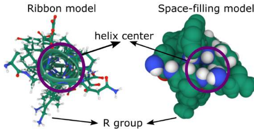
Figure 02-13: Different top-down views of a single alpha helix. Ribbon models of helices (shown on the left, with the R groups sticking out the “ribbon” path of the backbone) can give a false illusion that there is space inside the helix large enough for molecules to pass through. The space-filling model confirms that the internal area of the helix is filled by the space taken up by the atoms of the peptide backbone. This image is a derivative of 5EH6 created with NGL viewer by Dr. Lauren Dalton and is shared under a CC BY-SA 4.0 license.
