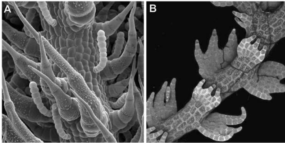
Figure 01-10: SEM versus fluorescence microscopy. (A) The lower surface of a sunflower leaf ( Helianthus annuus ) imaged by SEM. Attribution: Louisa Howard (2012), CIL:39342, https://doi.org/10.7295/W9CIL39342 . This image is in the public domain. (B) 3D reconstruction of the structure of the little fingers liverwort ( Lepidozia reptans ). This image was collected using fluorescence light microscopy by Dr. Robin Young and licensed under a CC BY-SA 4.0 license.
