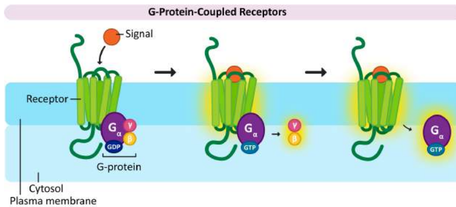
Figure 07-07: The activation of G-proteins. When a signal molecule binds, this activates the G-protein-coupled receptor. The activated receptor swaps out GDP for GTP on G_{\alpha} . When bound to GTP, the G_{\alpha} separates from G_{\beta\gamma} . These two molecules stimulate further downstream signaling. This image was created by Heather Ng-Cornish and is shared under a CC BY-SA 4.0 license.
