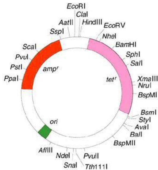
General structure of pBR322
