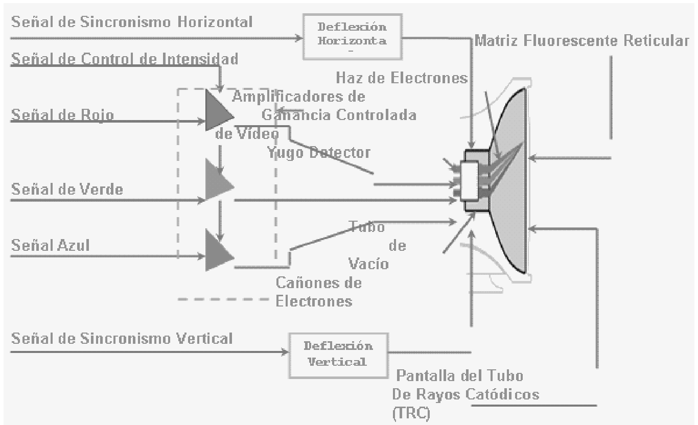
Figura 2.6: Pantalla CRT
