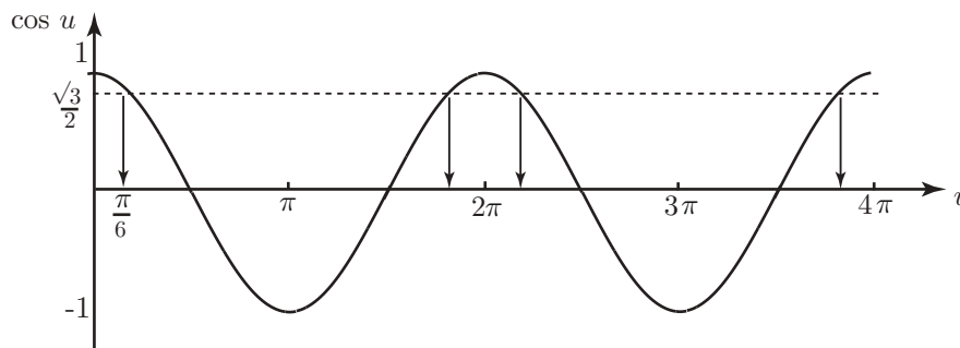
Figure 12. A graph of \cos u .
