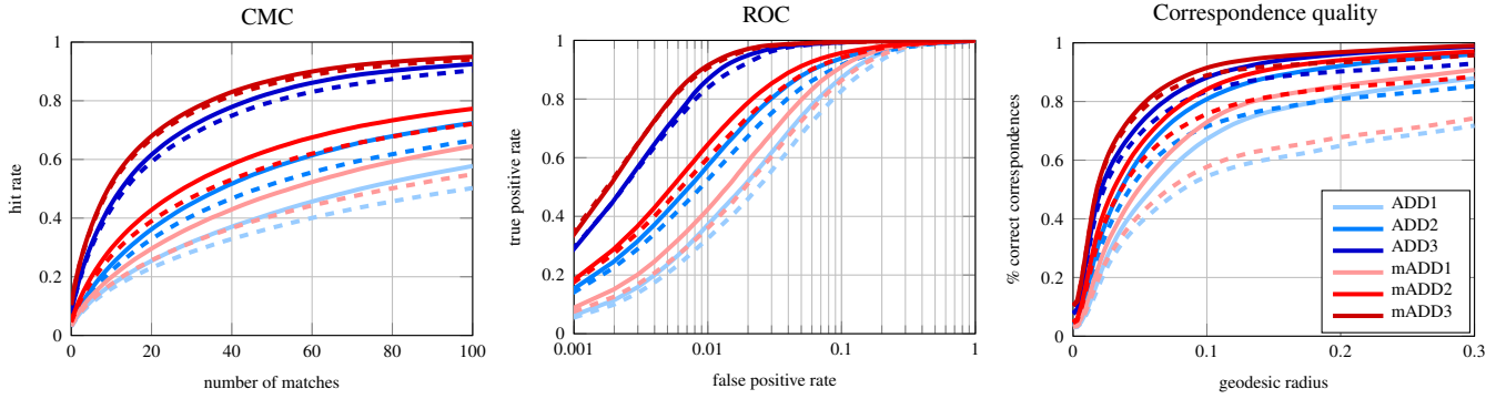
Figure 8: Performance of different architectures of our anisotropic descriptor measured using CMC (left), ROC (center) and Princeton protocol for nearest-neighbor correspondence (right); higher curves correspond to better performance. Shown are symmetric (solid) and asymmetric (dashed) settings. Training and testing were done on disjoint sets of the FAUST dataset.
