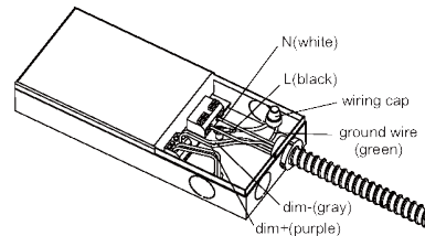
1. Replace the existing light fixture with the LED Light Panel.
