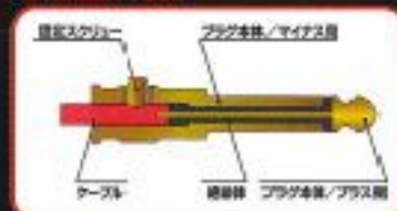
STRAIGHT PLUG
