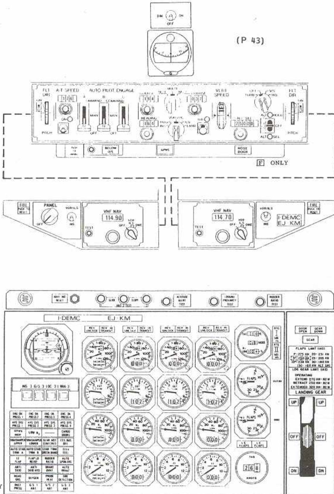
CENTER INSTRUMENT PANEL (P 2/P 33)
