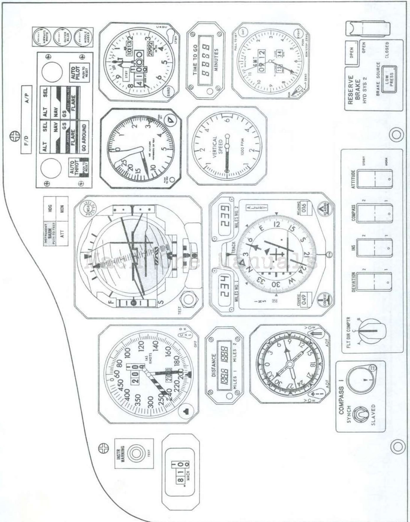
CAPTAIN'S INSTRUMENT PANEL
