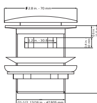
POP-UP DRAIN
