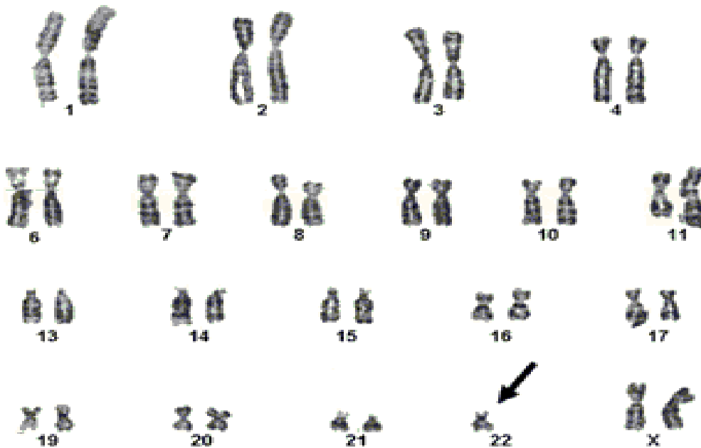
Monosomy – chromosome 22
