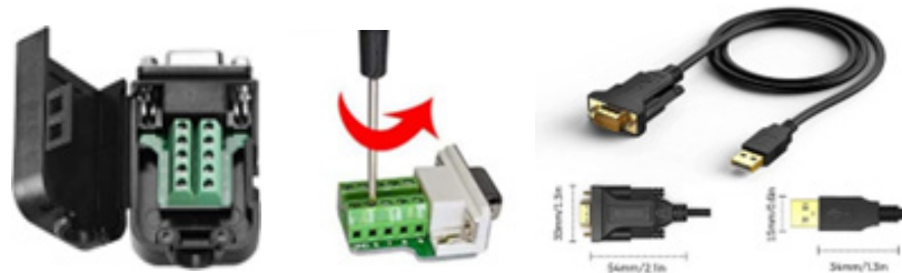
Reader Serial Port Service Kit
