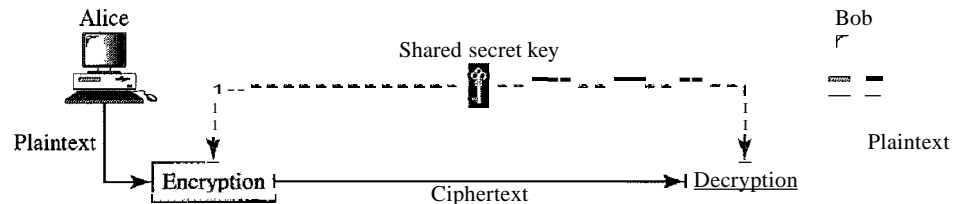
Figure 30.3 Symmetric-key cryptography
