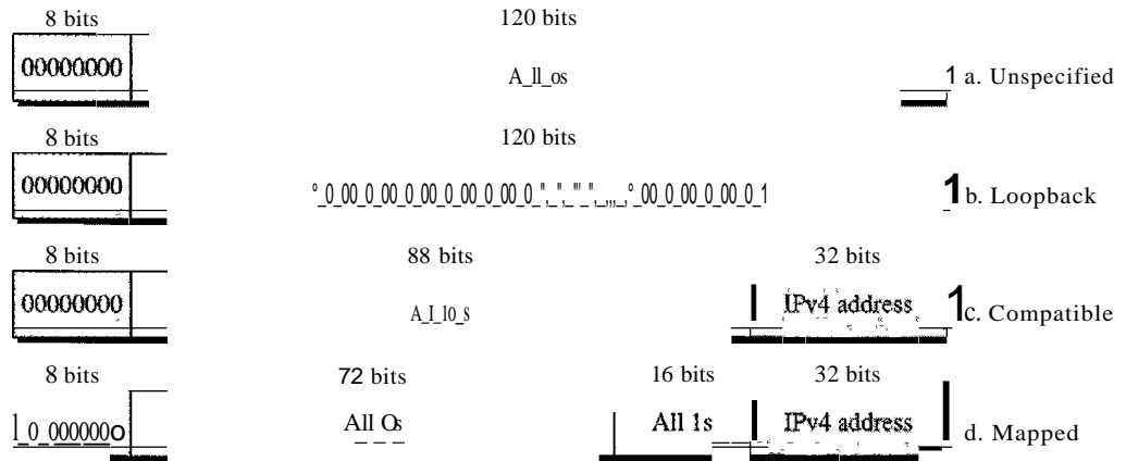
Figure 19.18 Reserved addresses in IPv6
