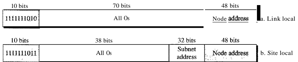
Figure 19.19 Local addresses in IPv6
