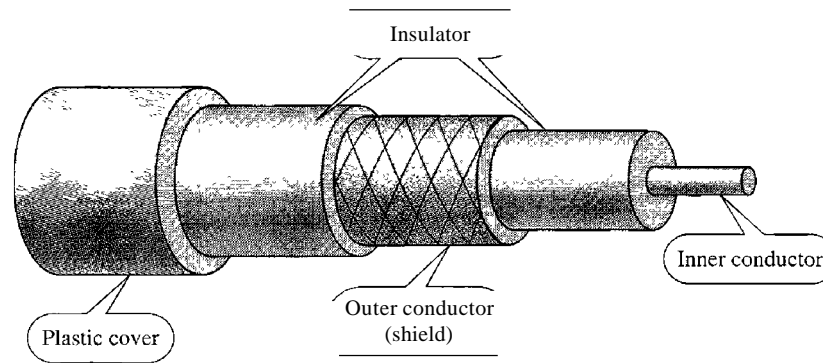
Figure 7.7 Coaxial cable
