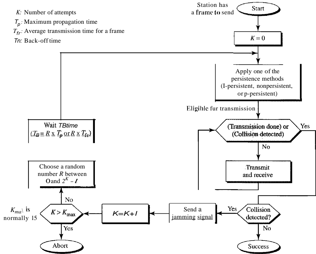
Figure 12.14 Flow diagram for the CSMA/CD
