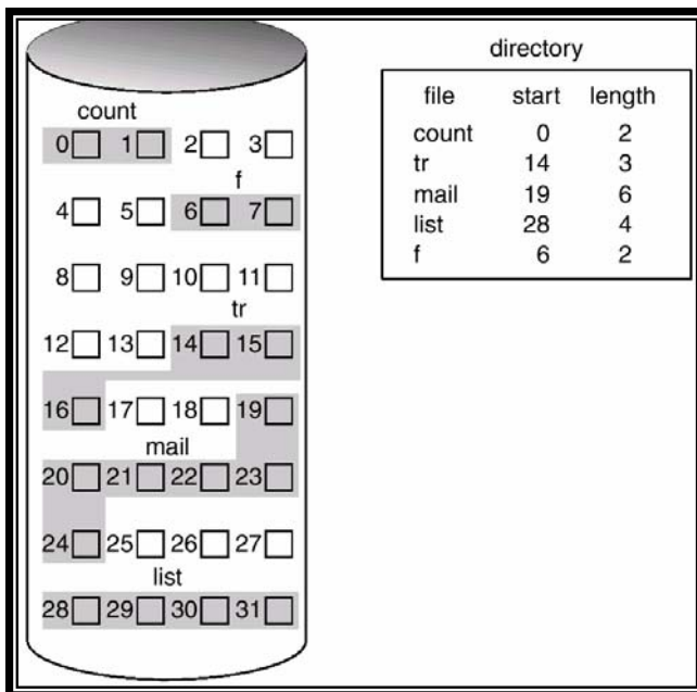
Contiguous allocation
