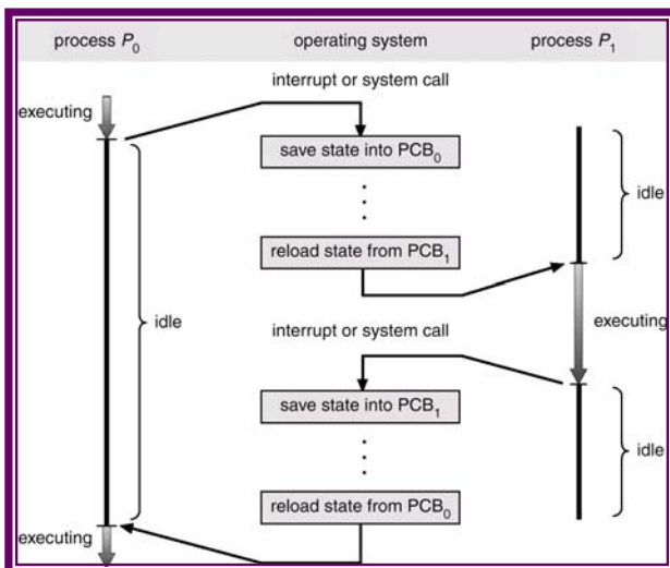
Figure 5.4 Context switching
