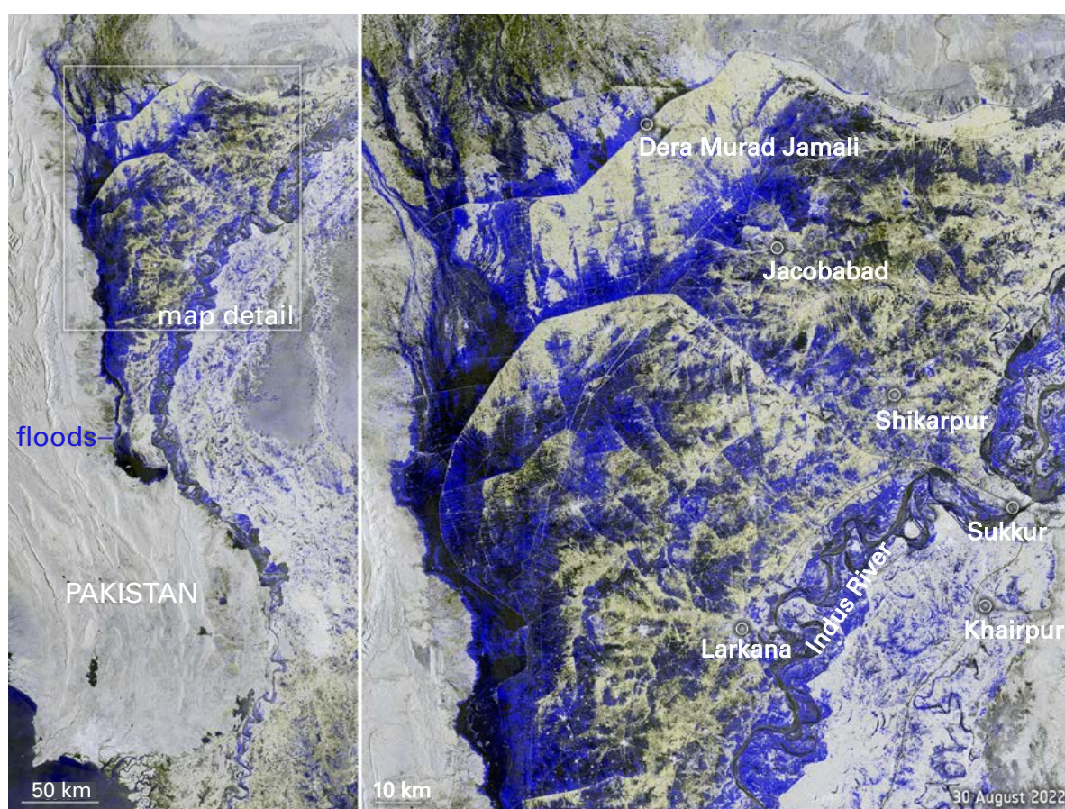
Figure 25. Satellite image of flooding in Pakistan on 30 August. The left side of the image shows a wide view of the area affected and the right side shows an enlarged view of the area between Dera Murad Jamali and Larkana. The blue to black colours show where the land is submerged.
