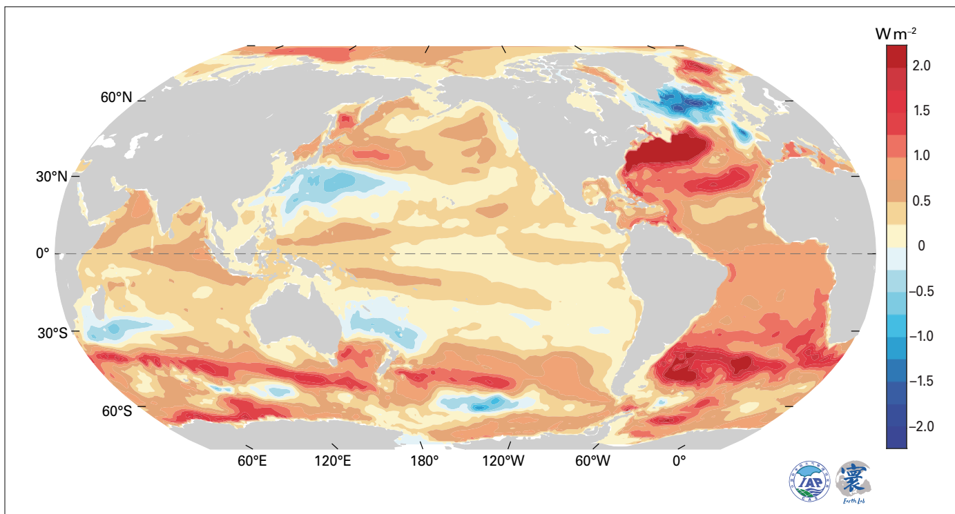
Figure 5. Estimated trend ( \text{W m}^{-2} ) in observed annual upper 2 000 m OHC from 1958 to 2022.
