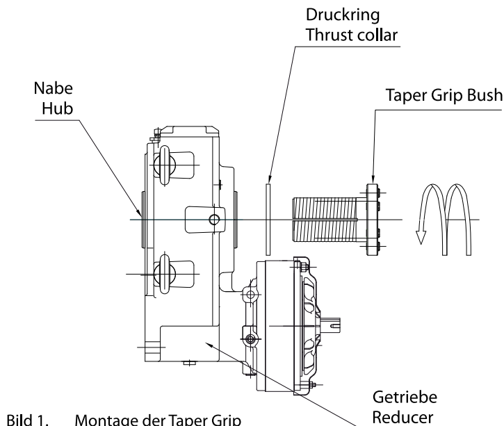
Bild 1. Montage der Taper Grip Figure 1. Bush Attachment to the Reducer
