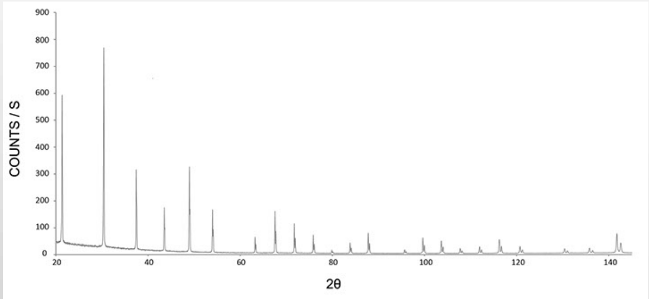
Scan of Lanthanum Hexaboride ( \text{LaB}_6 )
