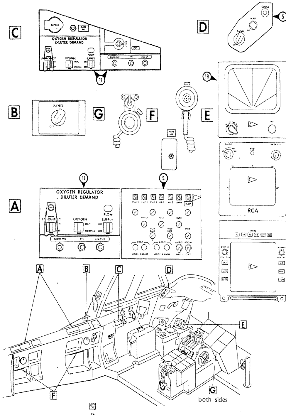
CAPTAIN & FIRST OFFICER'S AUXILIARY PANELS 2B5F 3B5
