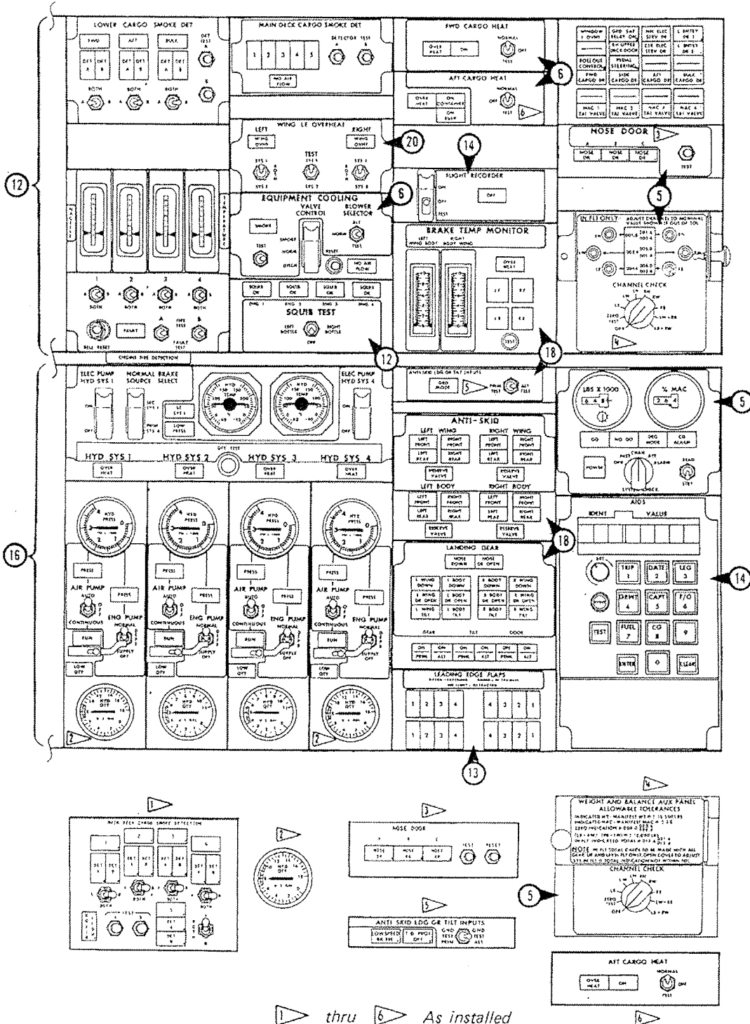
FLIGHT ENGINEER'S INSTRUMENT PANEL - UPPER PART - RIGHT 2B5F
