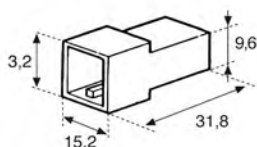
• 2-way male
