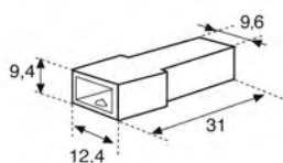
• 1 way male
