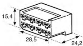
• 8 way female
