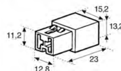
• 2 way female
