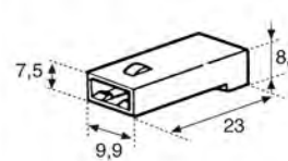
• 1 way female
