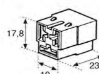
• 3 way female.
