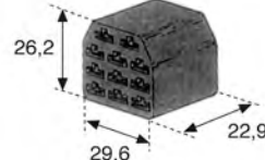
• 11 way female
