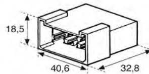
• 8-way male
