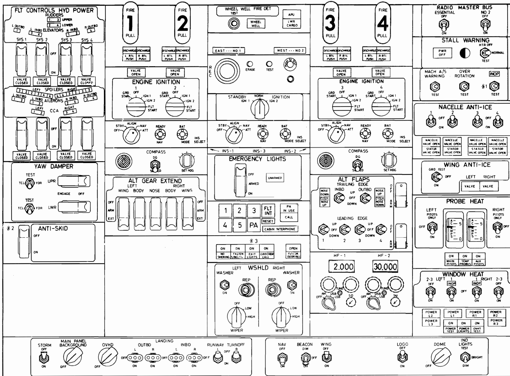
PILOTS' OVERHEAD PANEL
