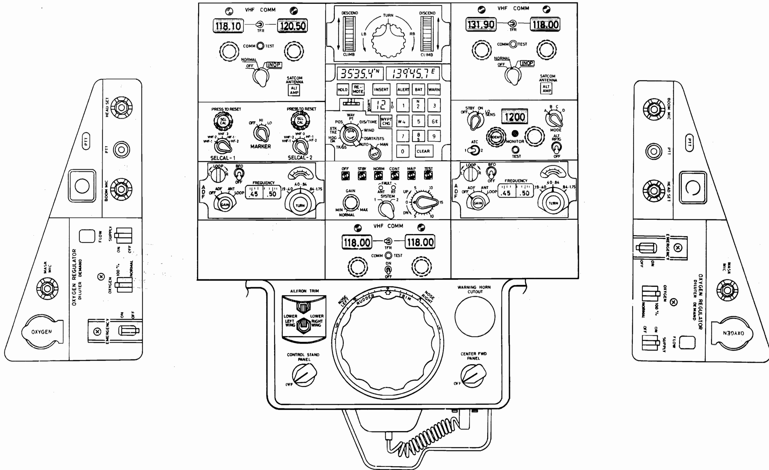
PILOTS' CONTROL STAND - AFT
