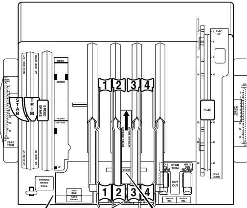
ENGINE START LEVERS
