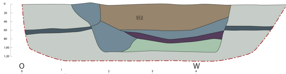
Coupe S20
