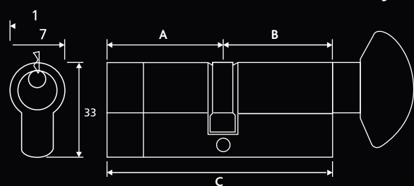
Fortress 3 Star BS Double Euro Profile Thumbturn Cylinder
