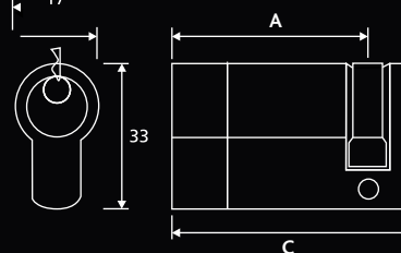
Fortress 3 Star BS Single Euro Profile Cylinder
