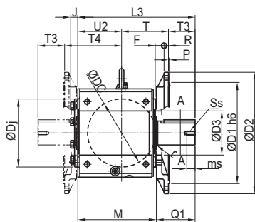
Solid Shaft 4F18DA~4F19DB
