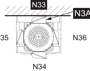
Mounting Positions Y5,G5
