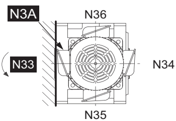
Mounting Positions Y2,G2,V2
