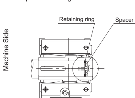
Secured by a spacer and stopper ring
