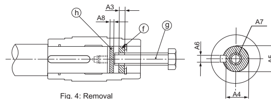
Fig. 4: Removal
