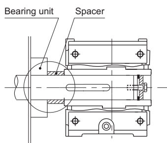
Secured by a spacer (non stepped driven shaft)
