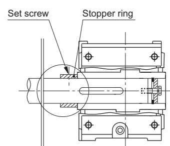
Secured by a set screw and stopper (non stepped driven shaft)
