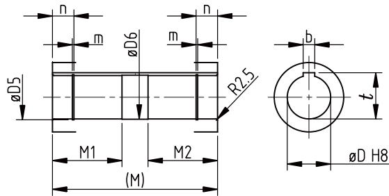
A-A (Hollow Bore Shaft)
