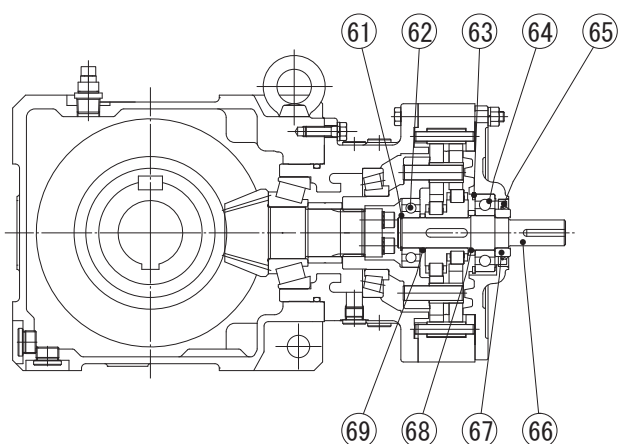
Fig. 2 Reducer
