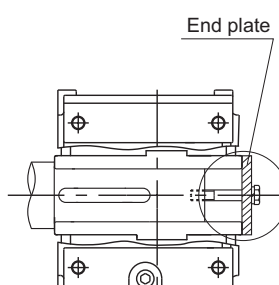
Secured by an end plate
