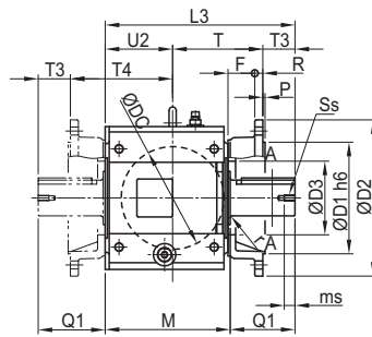
Solid Shaft 4A10□~4E19□
