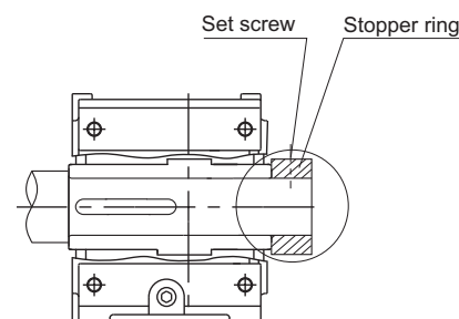
Secured by set screw and stopper ring
