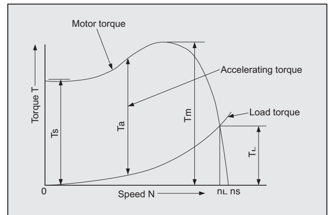
Torque Curve T_s : Starting torque
