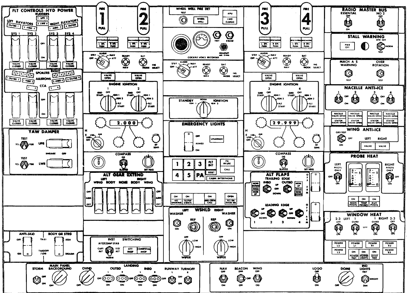
PILOT'S OVERHEAD PANEL
