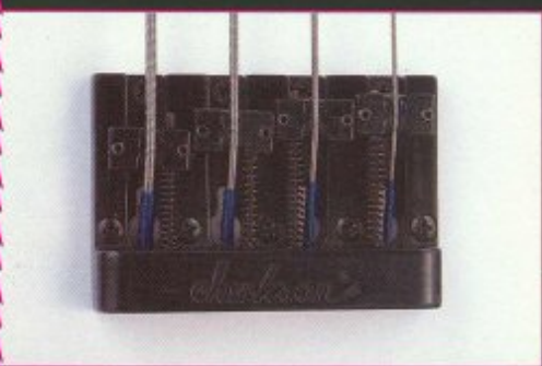
JB-440 HIGH DENSITY BRIDGE
