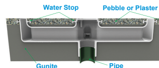
Unique water stop protects against leaks
