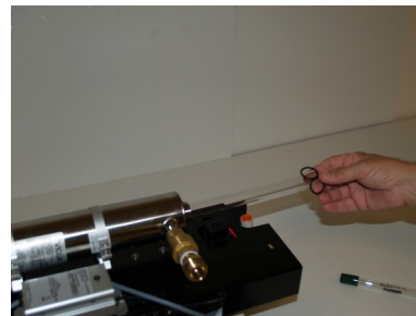
Remove quartz sleeve
