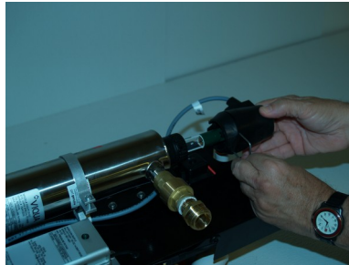
Remove bulb socket
