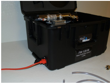
Connect 120v power
